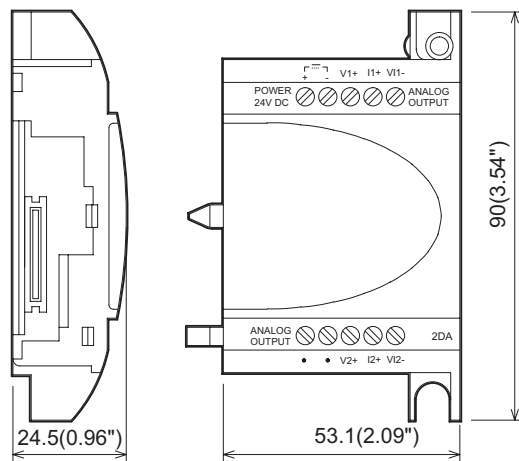
Figure 11.2: External Dimensions
