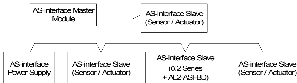
Figure 9.2: System Configuration
