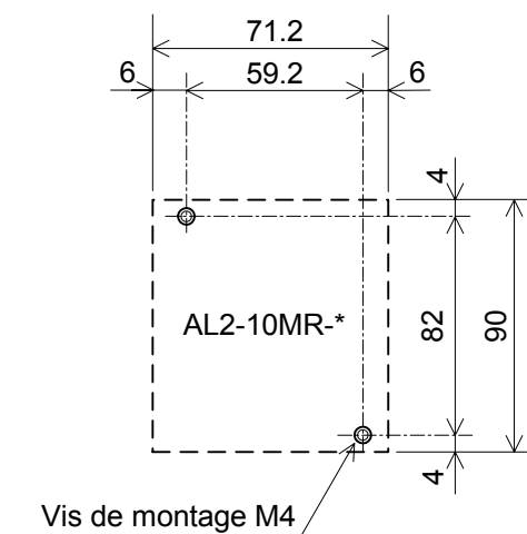
Figure 3.4: Montage direct
